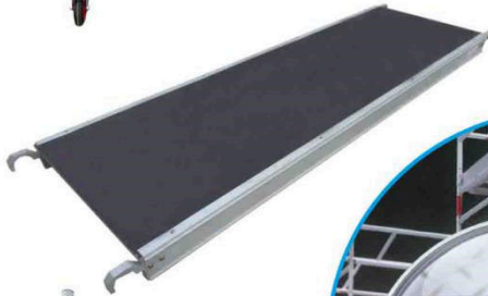
T10 L:1960xW740xH1940 Solid wheel:6" ① □30X151.2mm ②③ Φ50x1.6mm ④ 80x50x2mm
